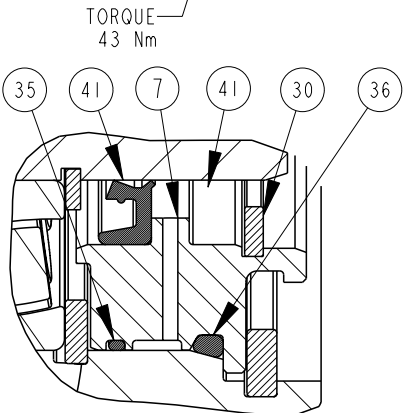
DUAL SHAFT SEAL ASSEMBLY P2-105-0210-02 SECTION A-A SCALE 1:1
